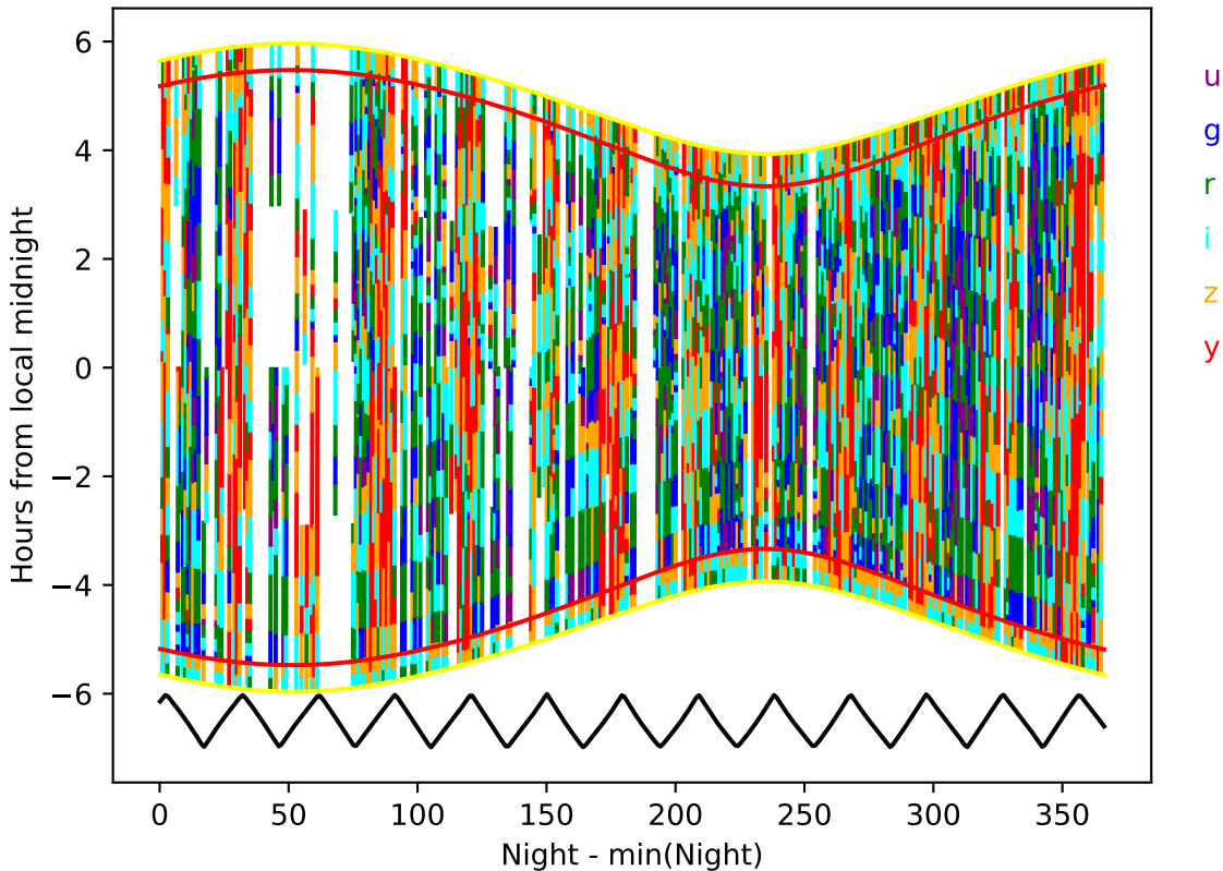
reweight_plane_v3.3_10yrs year 9-10: Hourglass
