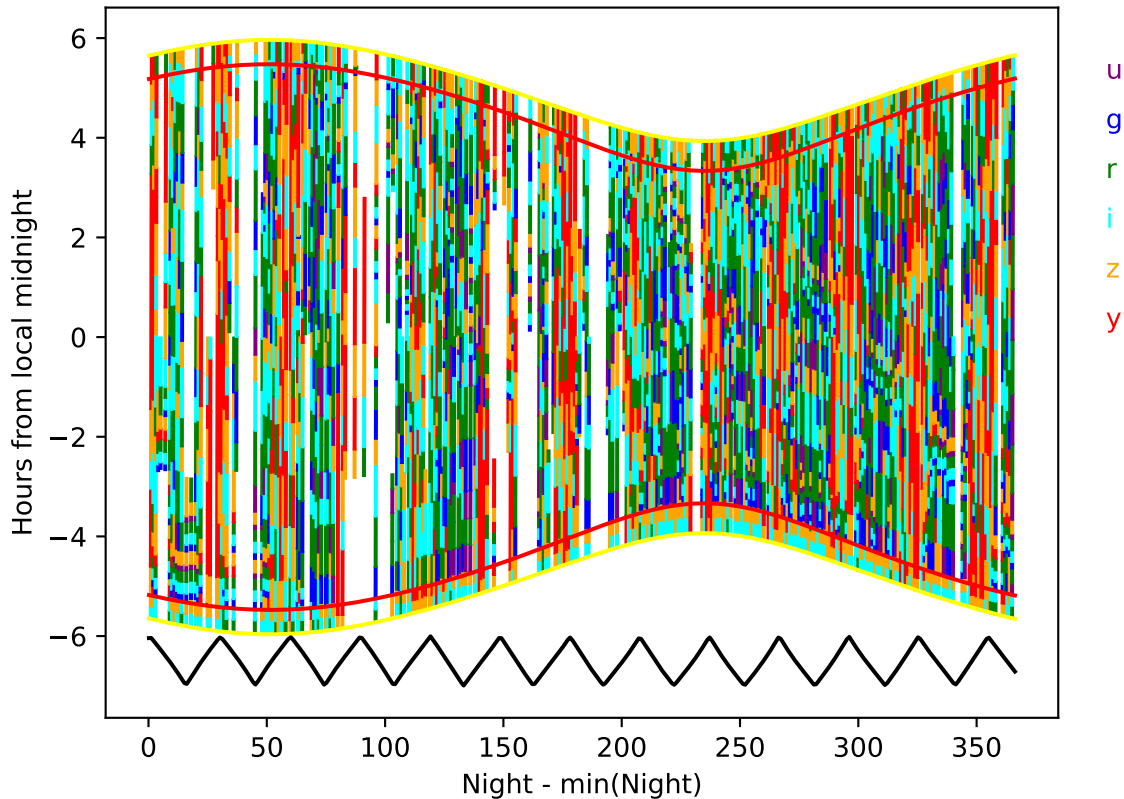
reweight_plane_v3.3_10yrs year 1-2: Hourglass
