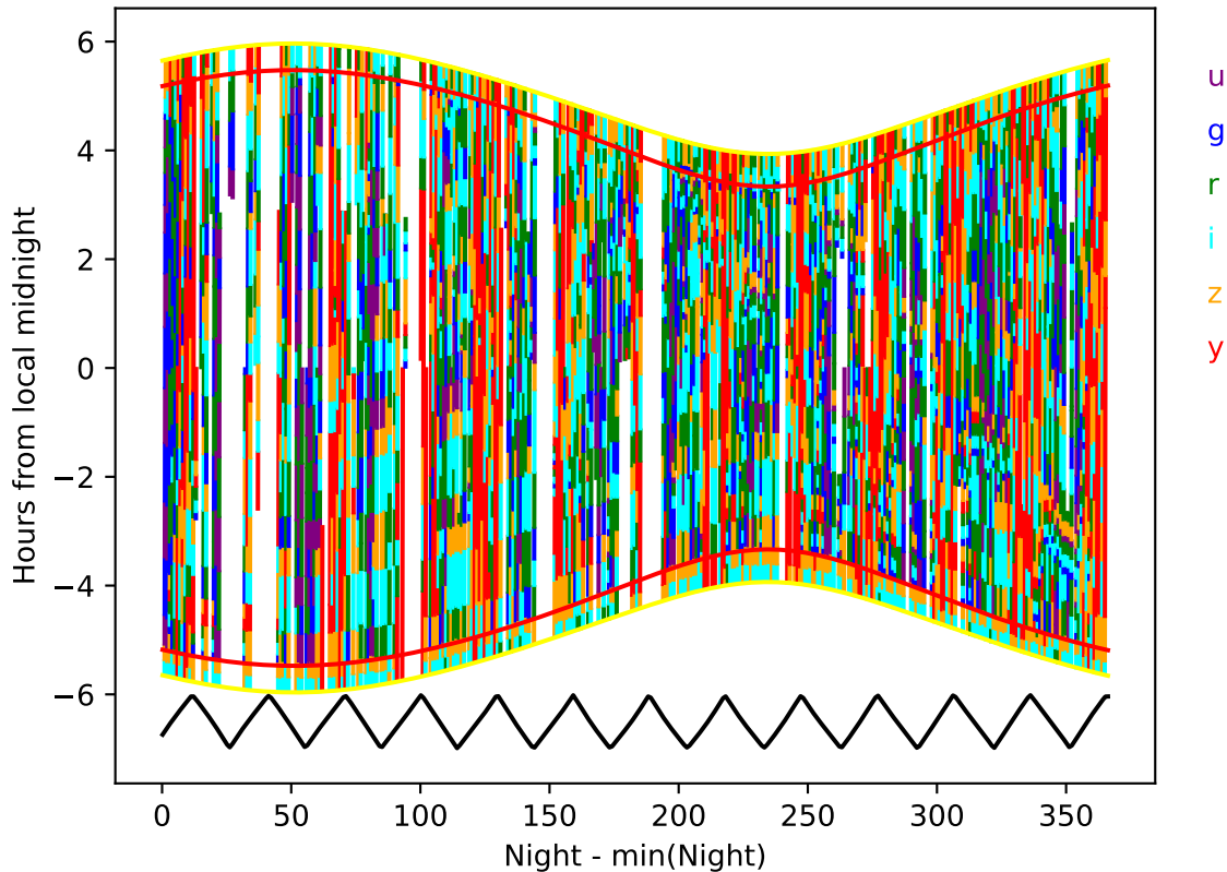
reweight_plane_v3.3_10yrs year 0-1: Hourglass
