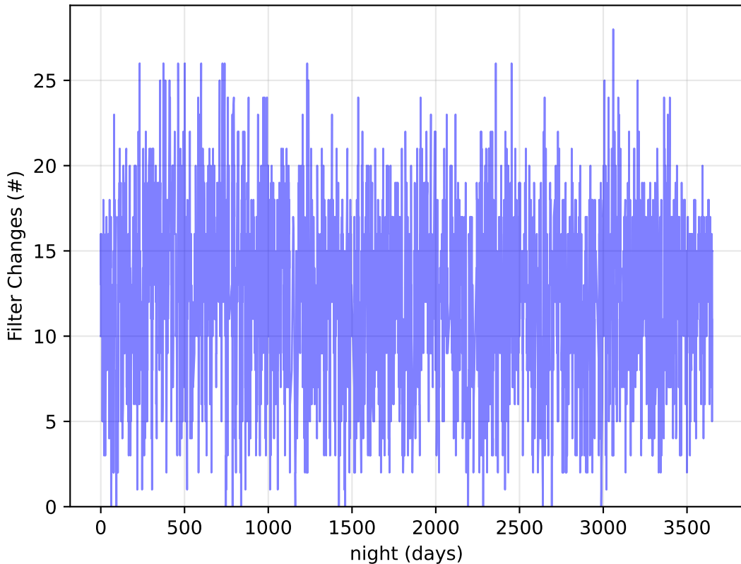
reweight_plane_v3.3_10yrs : Filter Changes
