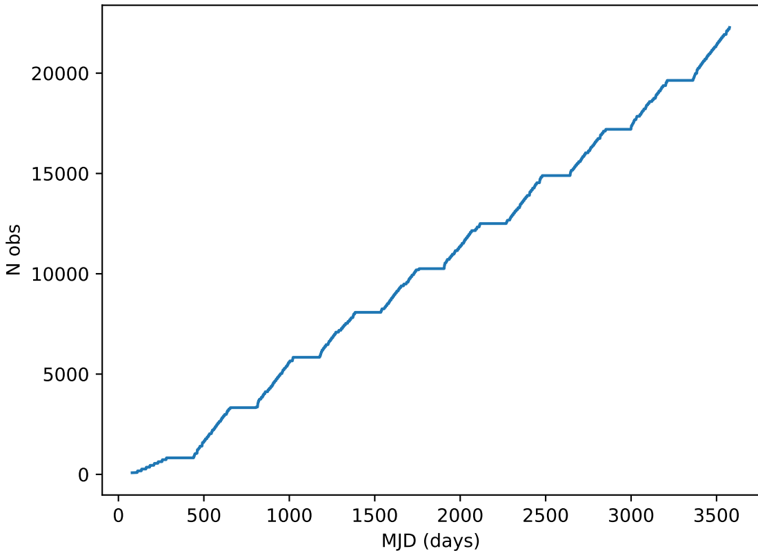
reweight_plane_v3.3_10yrs note like DD:XMM_LSS%: Cumulative
