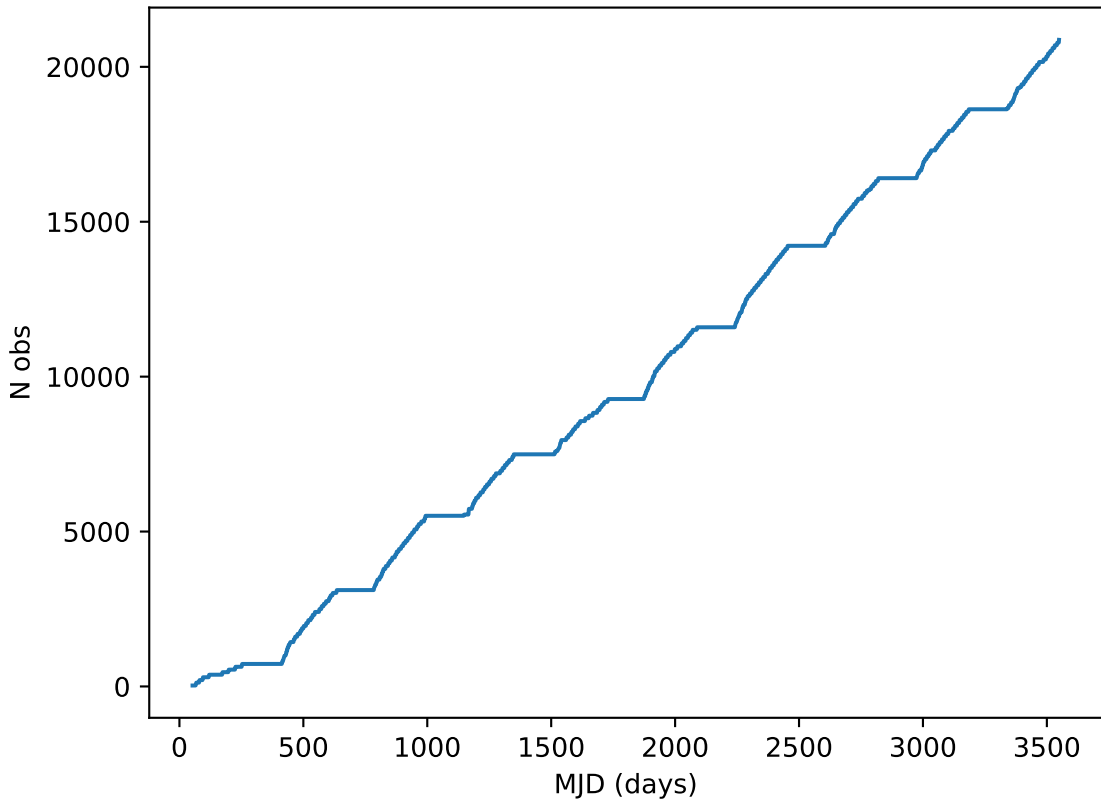
reweight_plane_v3.3_10yrs note like DD:ELAISS1%: Cumulative
