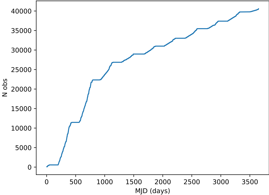
reweight_plane_v3.3_10yrs note like DD:COSMOS%: Cumulative
