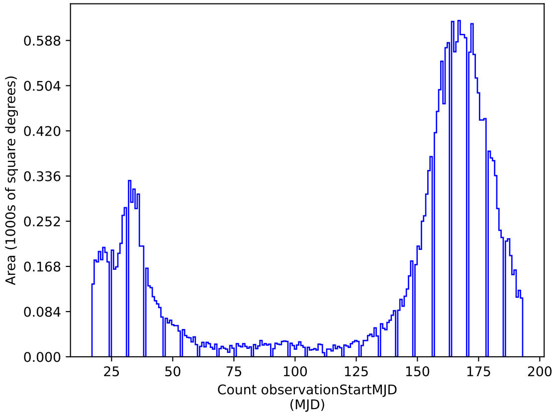
reweight_plane_v3.3_10yrs z: Count observationStartMJD
