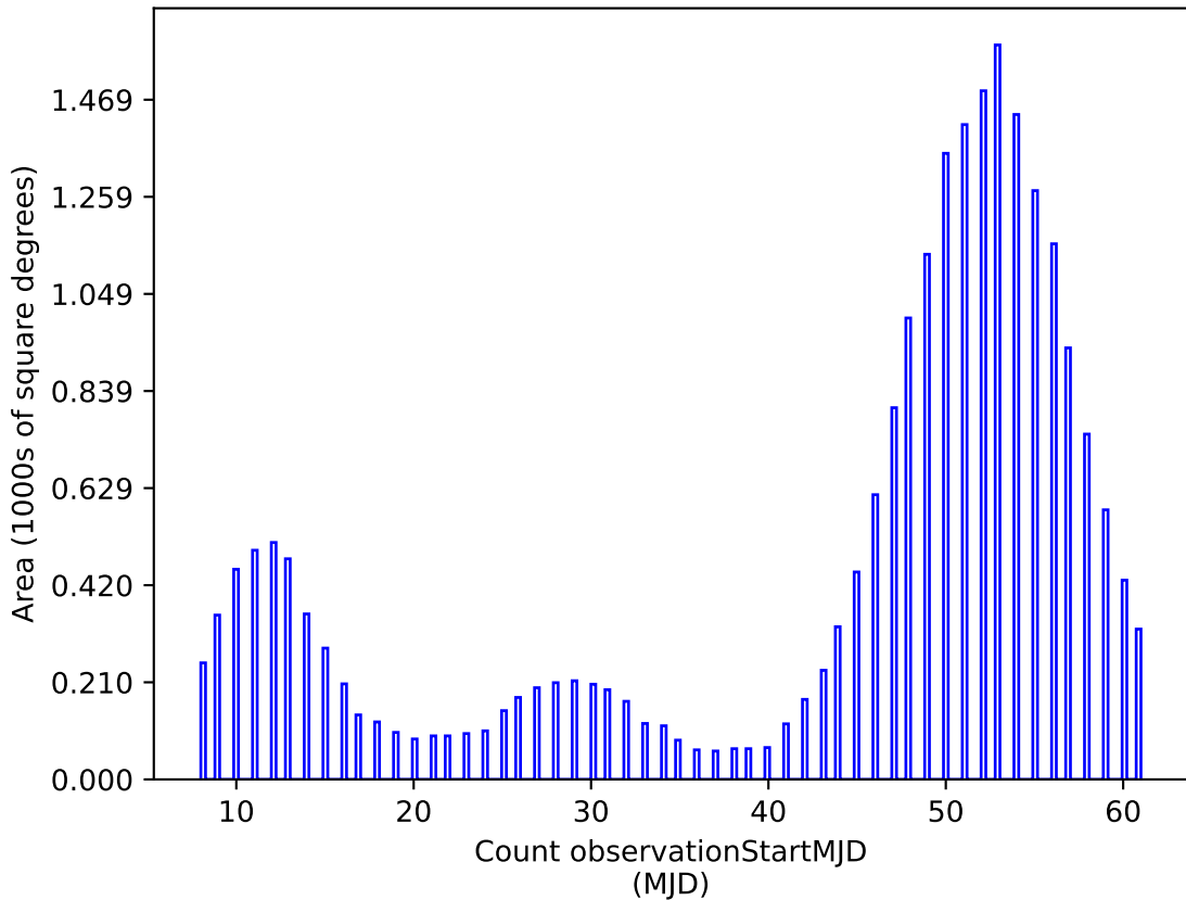
reweight_plane_v3.3_10yrs u: Count observationStartMJD
