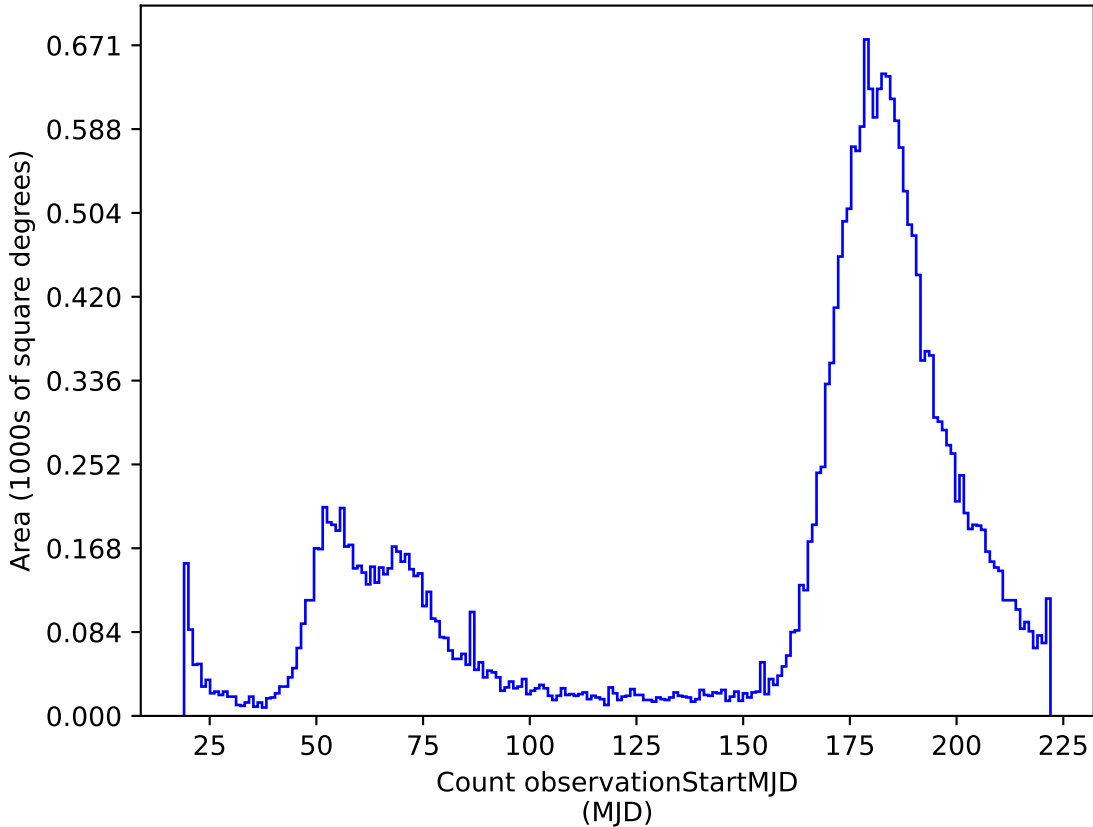
reweight_plane_v3.3_10yrs r: Count observationStartMJD
