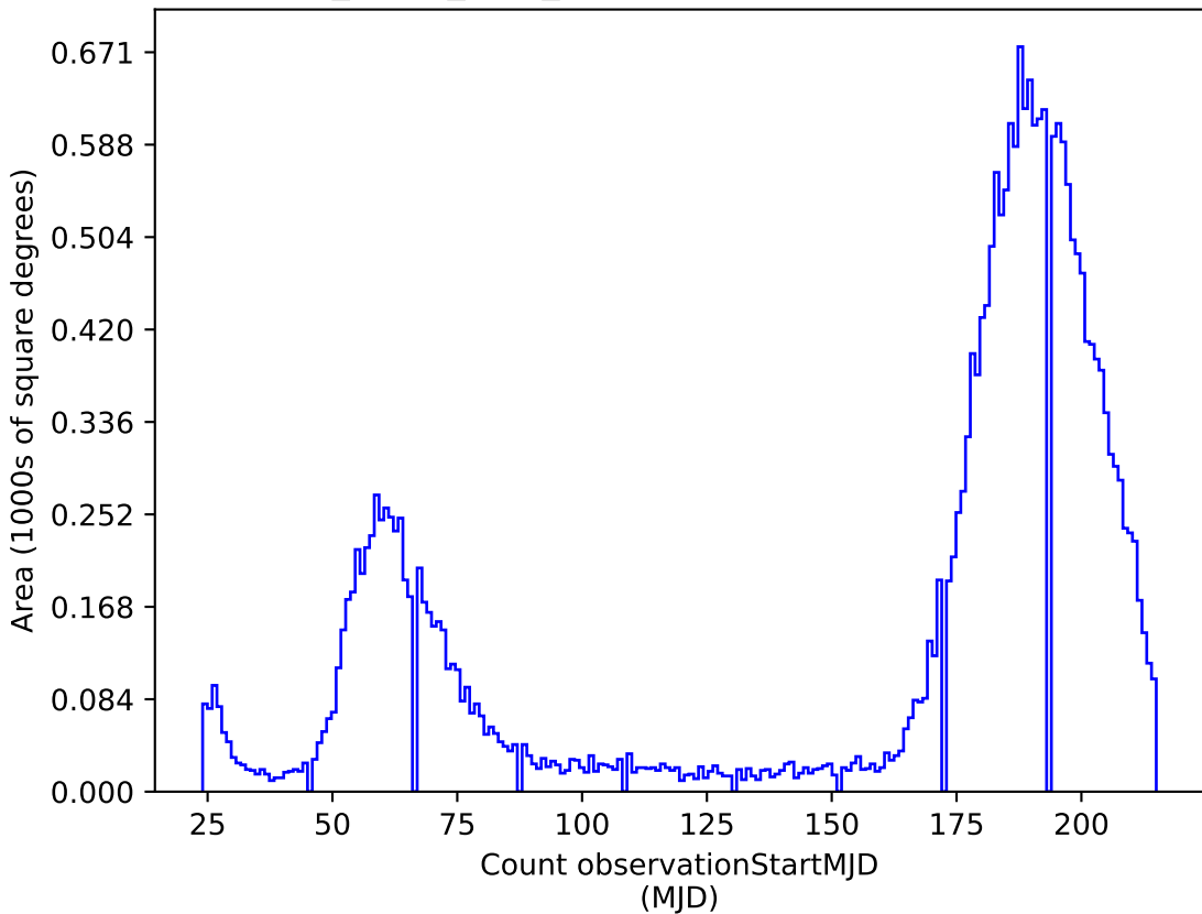
reweight_plane_v3.3_10yrs i: Count observationStartMJD
