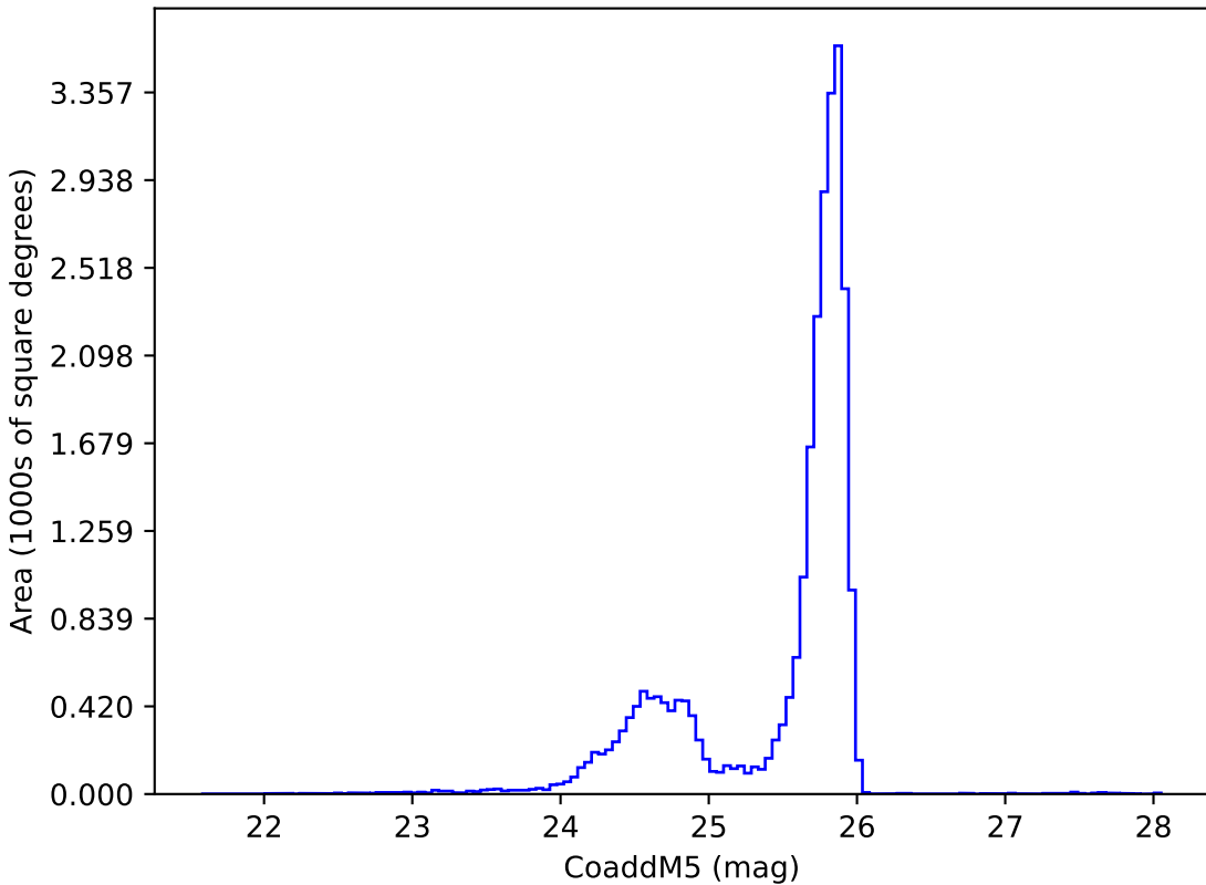
reweight_plane_v3.3_10yrs z: CoaddM5
