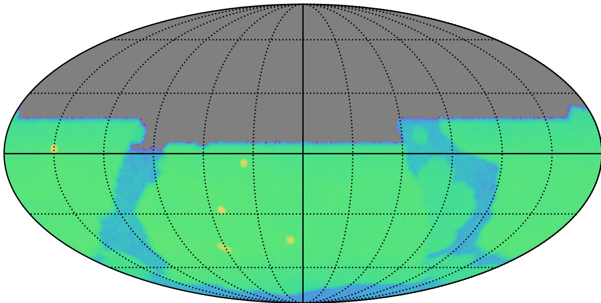
reweight_plane_v3.3_10yrs y: CoaddM5
