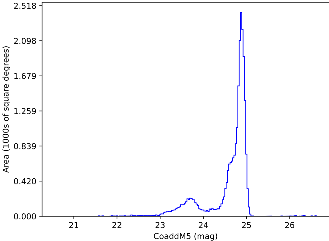
reweight_plane_v3.3_10yrs y: CoaddM5
