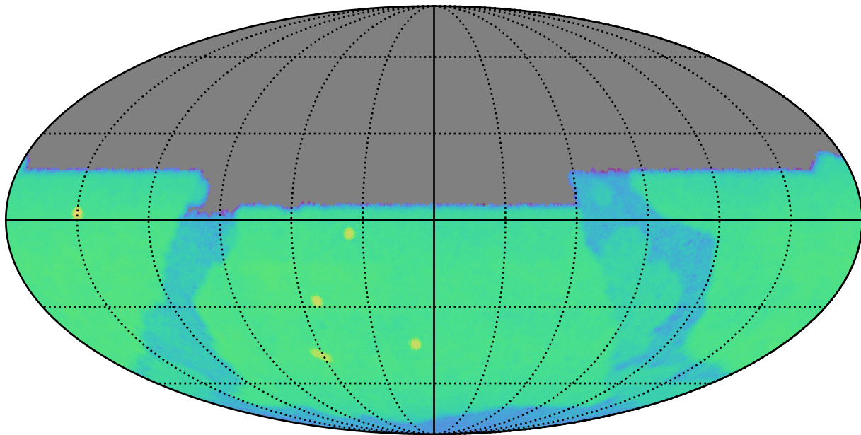
reweight_plane_v3.3_10yrs u: CoaddM5
