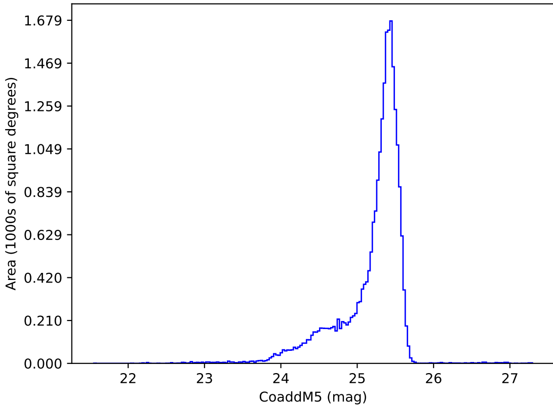
reweight_plane_v3.3_10yrs u: CoaddM5
