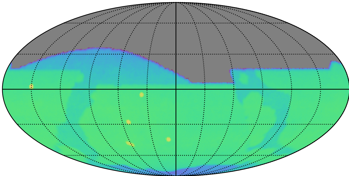
reweight_plane_v3.3_10yrs r: CoaddM5
