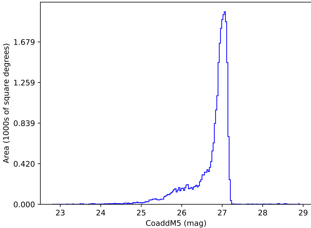
reweight_plane_v3.3_10yrs r: CoaddM5
