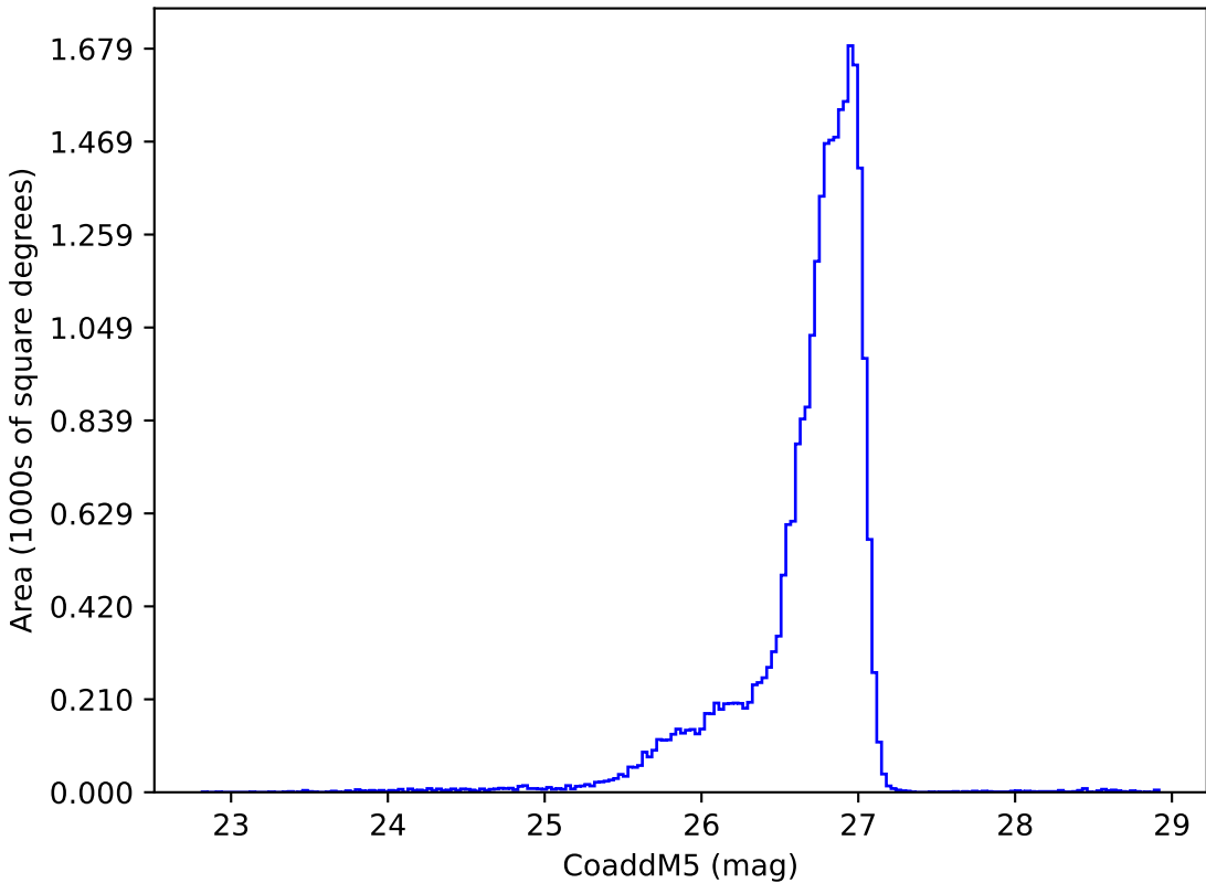
reweight_plane_v3.3_10yrs g: CoaddM5
