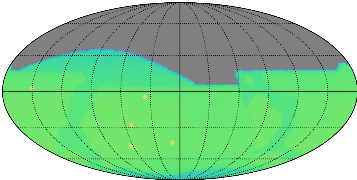
reweight_plane_v3.3_10yrs : CoaddM5
