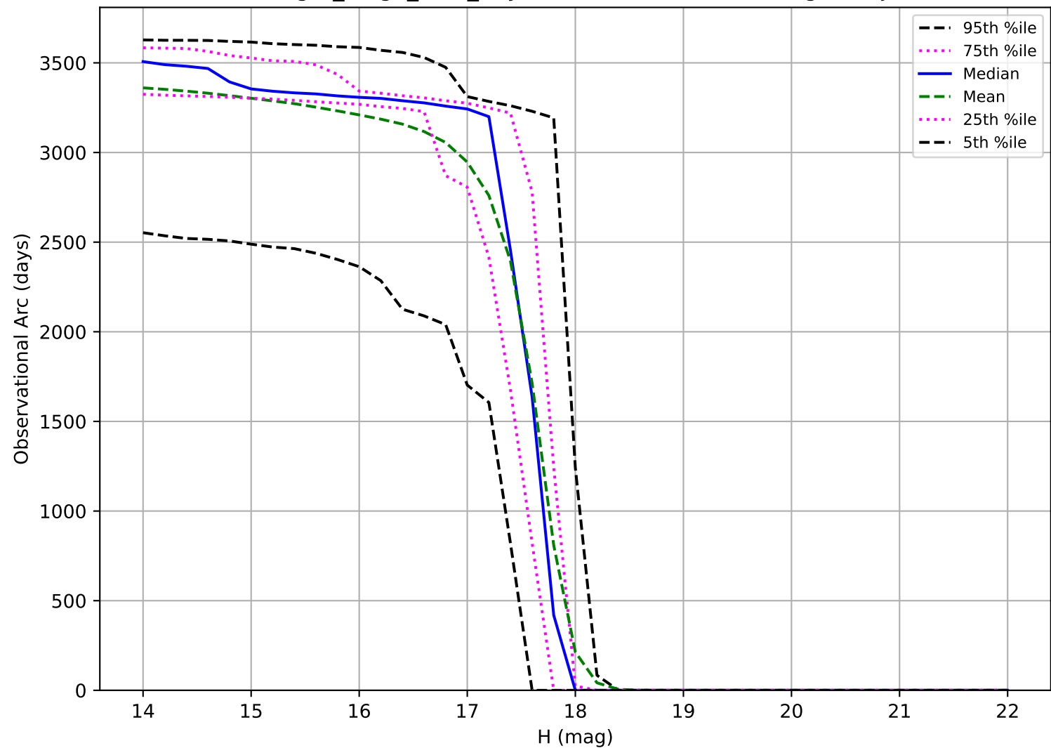
reweight_bulge_v3.3_10yrs: Observational Arc Length Trojan
