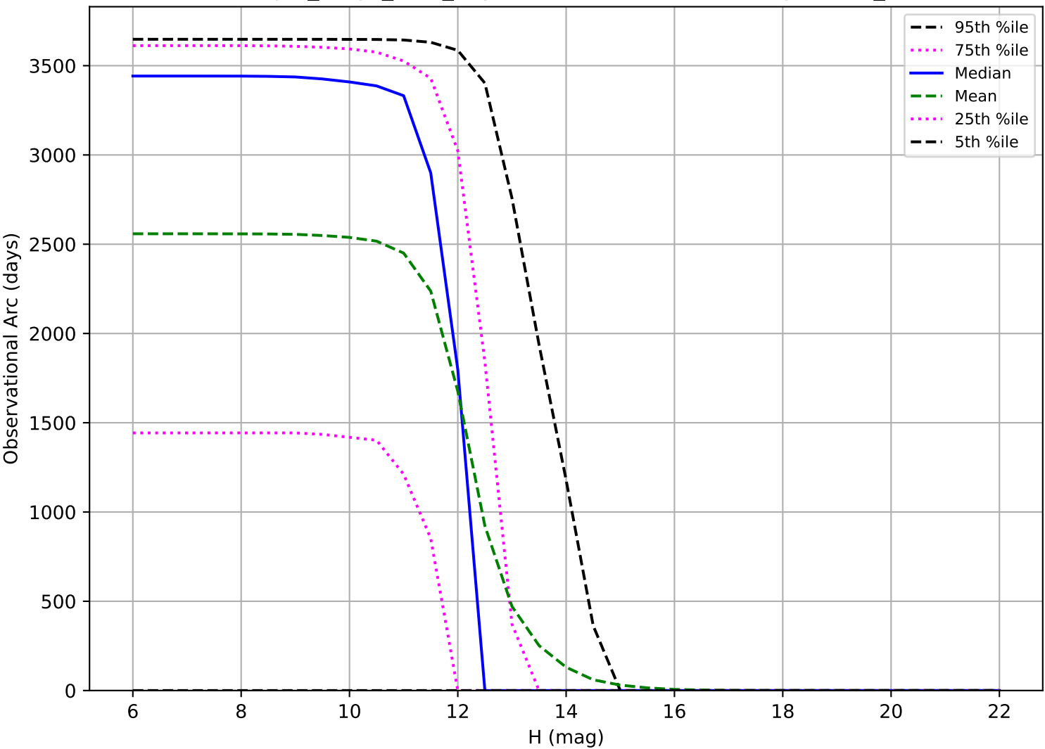
reweight_bulge_v3.3_10yrs: Observational Arc Length OCC_r20
