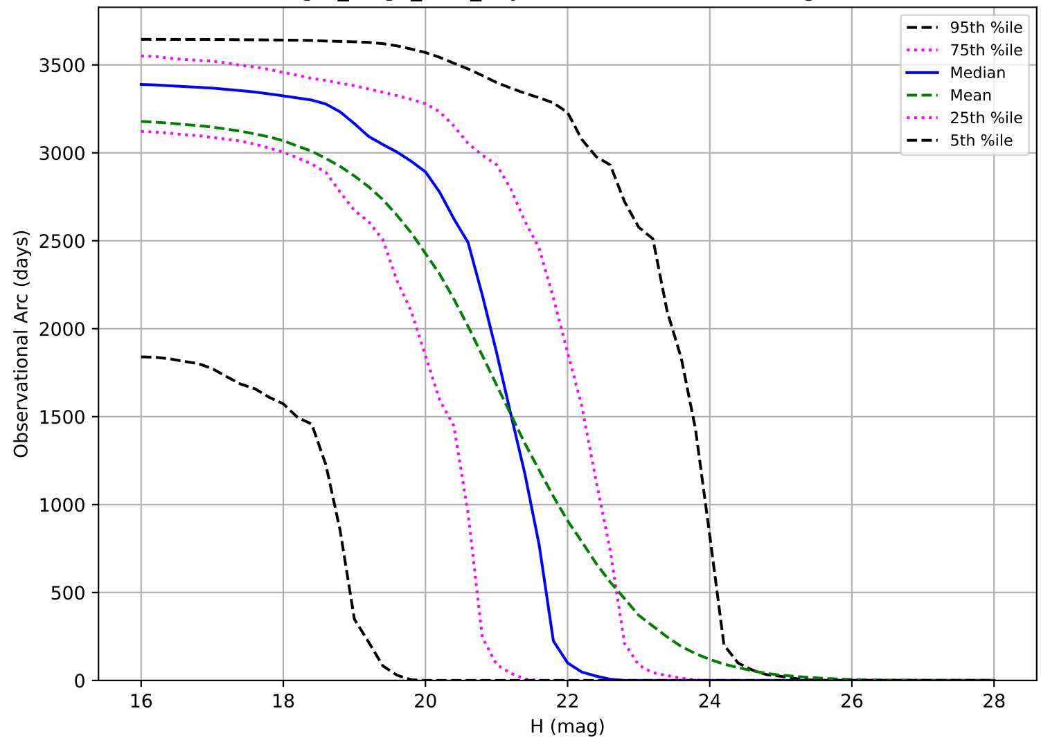
reweight_bulge_v3.3_10yrs: Observational Arc Length NEO
