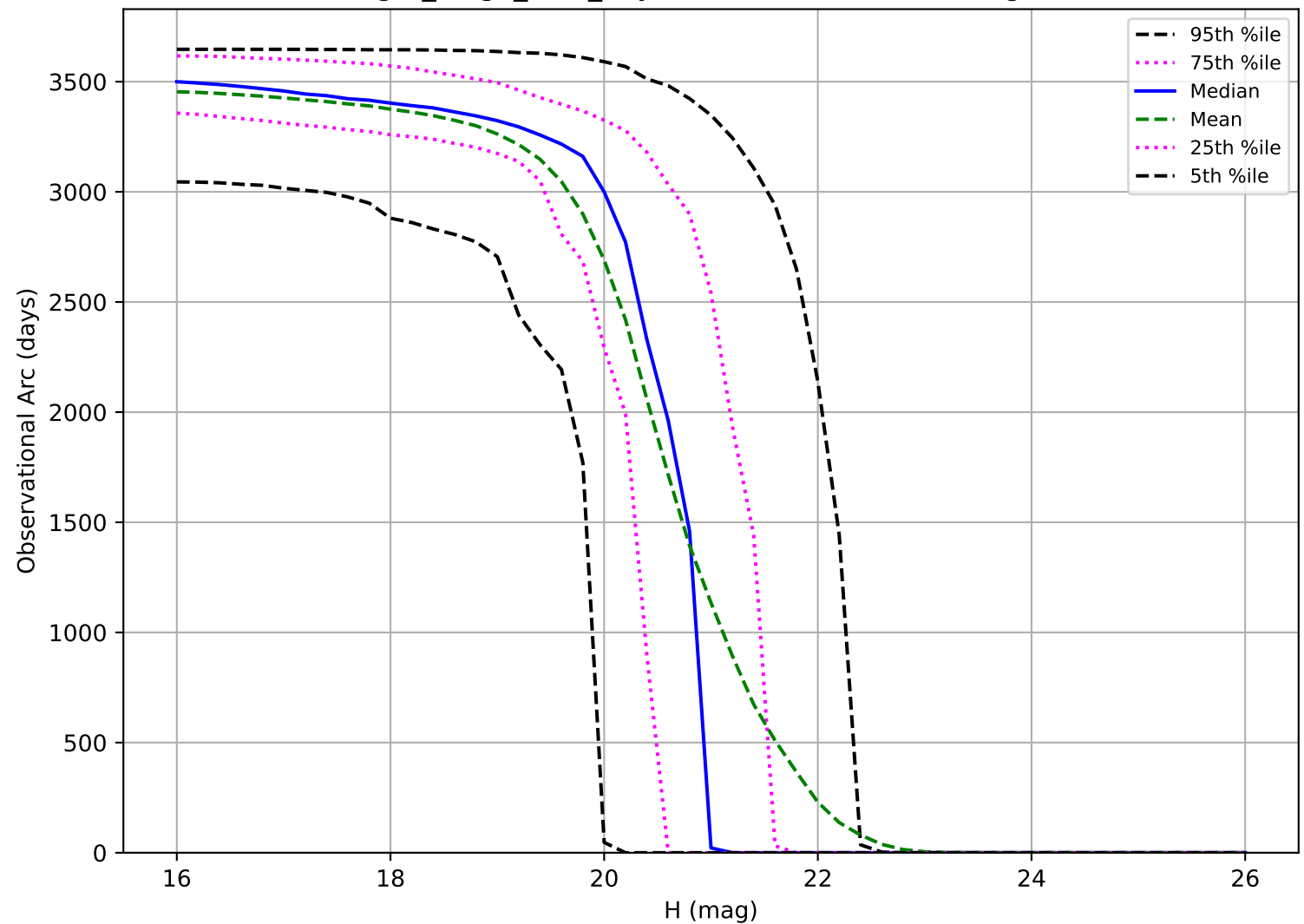
reweight_bulge_v3.3_10yrs: Observational Arc Length MBA
