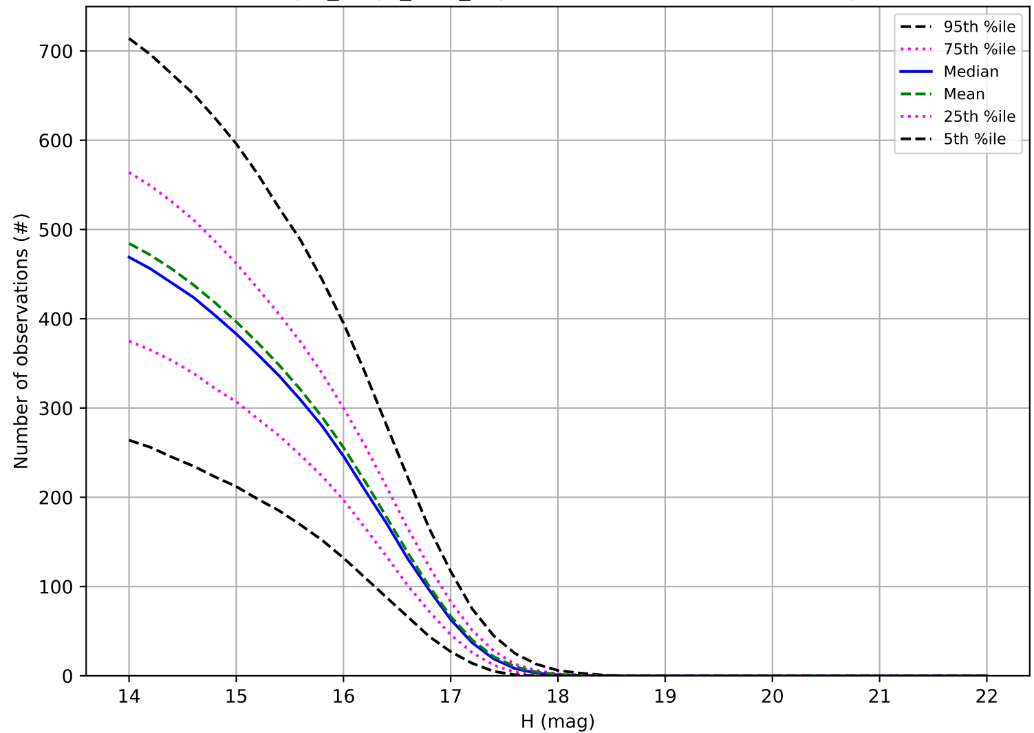
reweight_bulge_v3.3_10yrs: Number of observations Trojan
