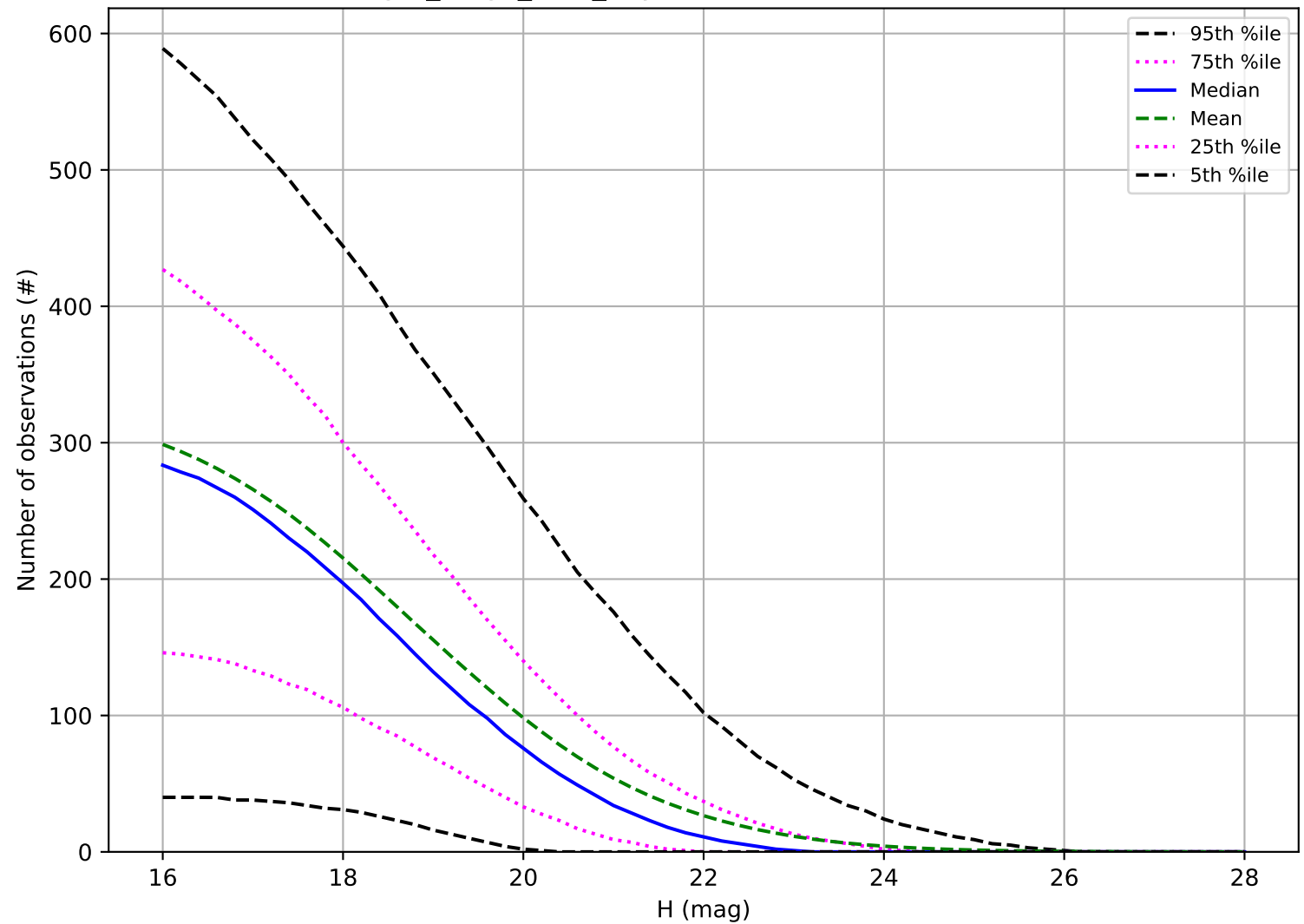
reweight_bulge_v3.3_10yrs: Number of observations PHA
