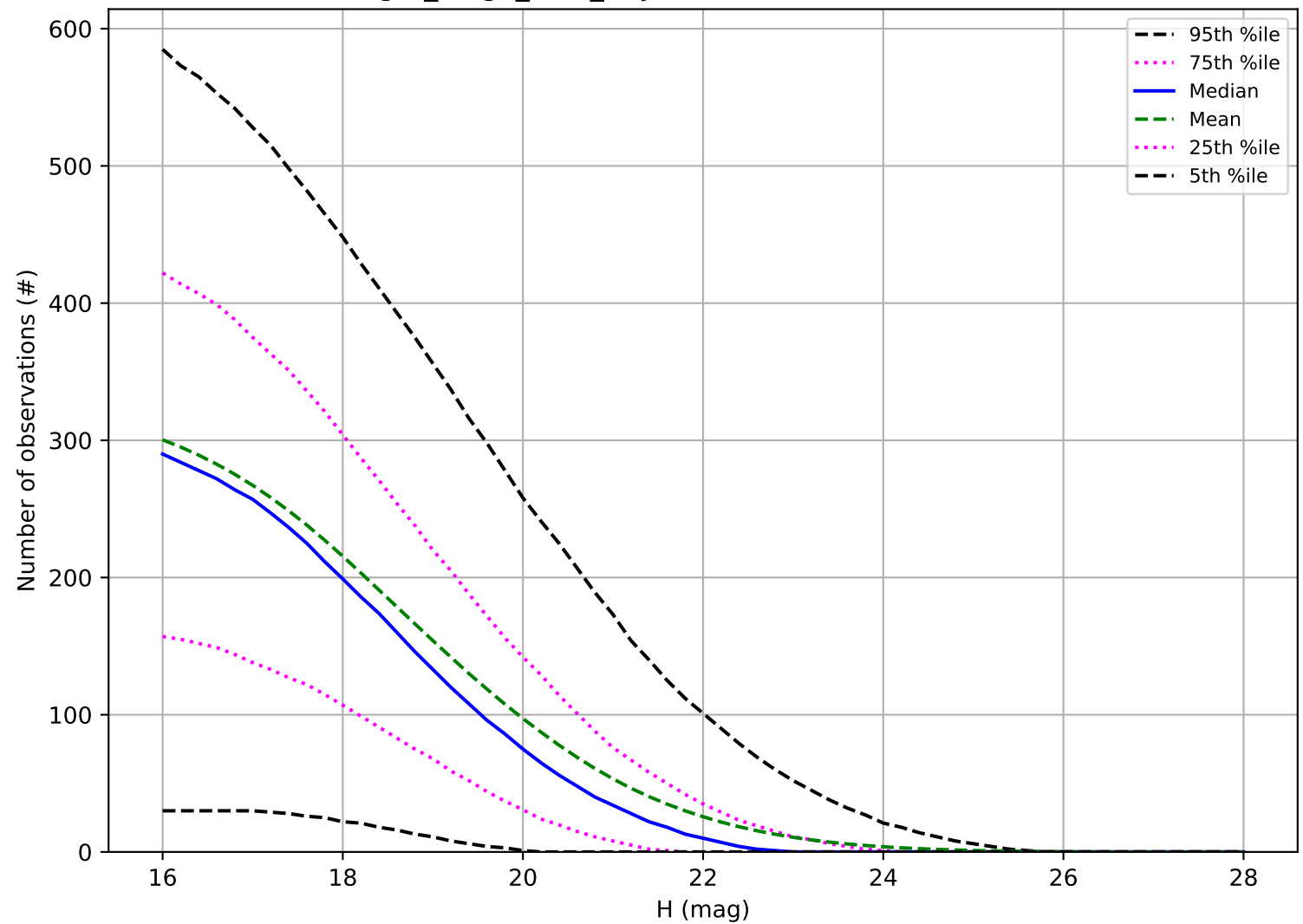
reweight_bulge_v3.3_10yrs: Number of observations NEO
