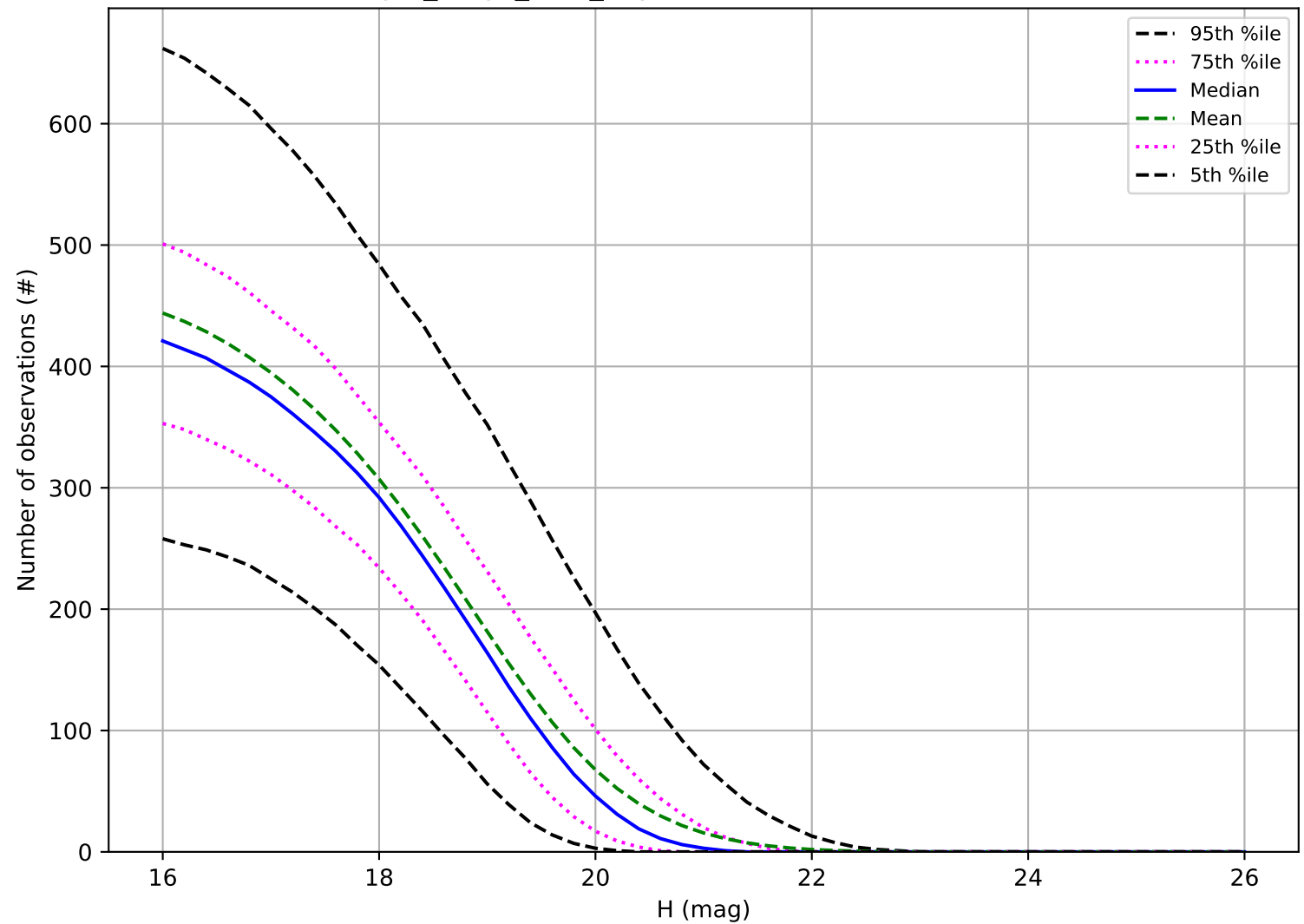
reweight_bulge_v3.3_10yrs: Number of observations MBA
