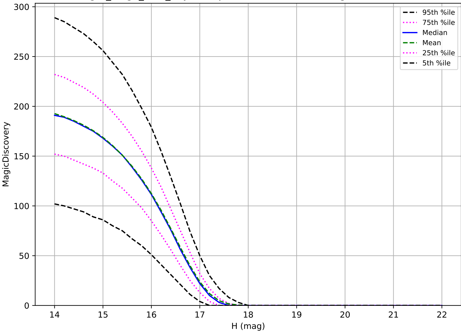
reweight_bulge_v3.3_10yrs: Trojan 6 detections in 60 nights detection loss
