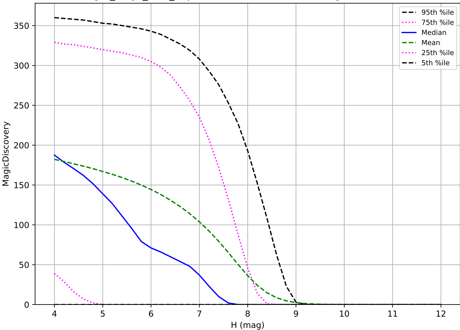
reweight_bulge_v3.3_10yrs: TNO 6 detections in 60 nights detection loss
