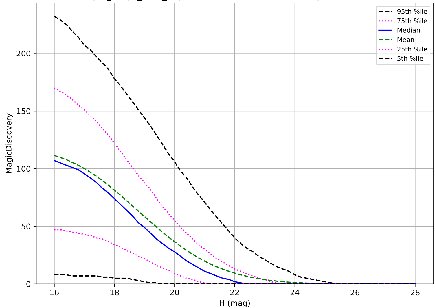
reweight_bulge_v3.3_10yrs: PHA 6 detections in 60 nights detection loss
