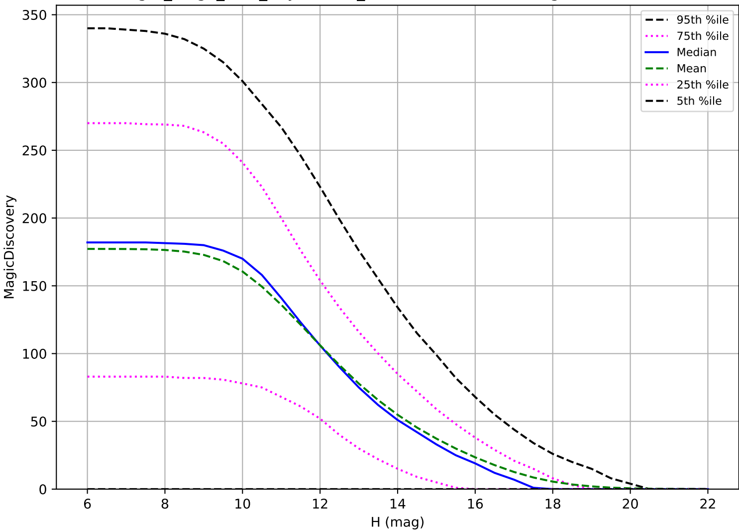
reweight_bulge_v3.3_10yrs: OCC_r5 6 detections in 60 nights detection loss
