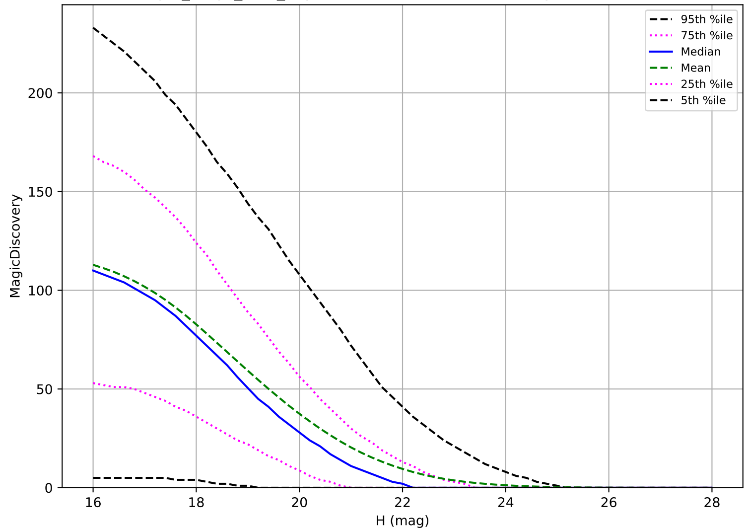
reweight_bulge_v3.3_10yrs: NEO 6 detections in 60 nights detection loss
