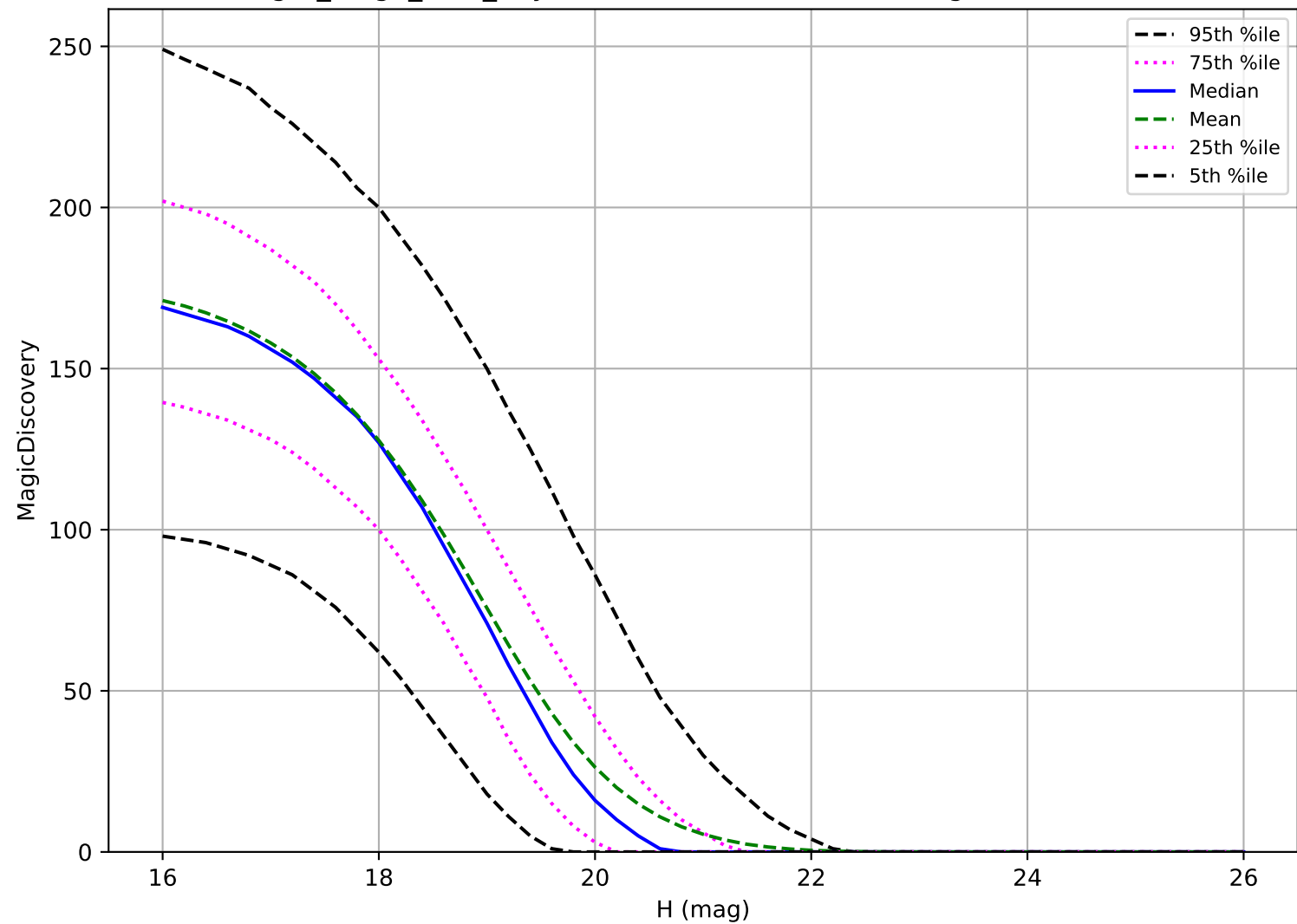
reweight_bulge_v3.3_10yrs: MBA 6 detections in 60 nights detection loss
