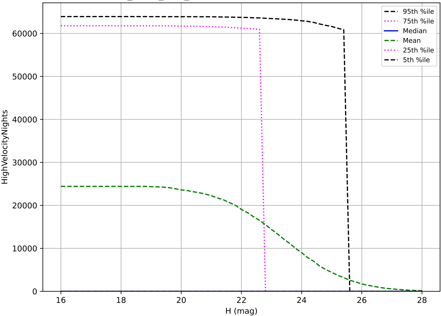
reweight_bulge_v3.3_10yrs: PHA High velocity pair detection loss
