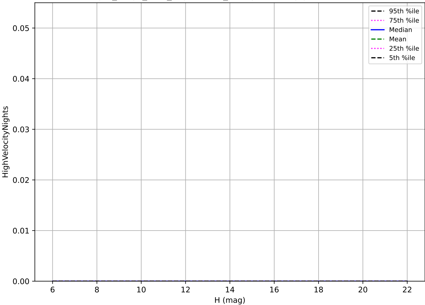
reweight_bulge_v3.3_10yrs: OCC_r5 High velocity pair detection loss
