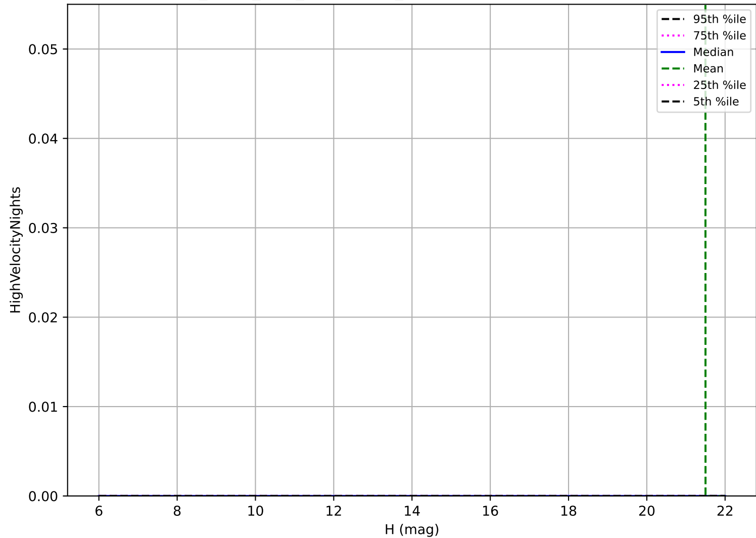
reweight_bulge_v3.3_10yrs: OCC_r20 High velocity pair detection loss
