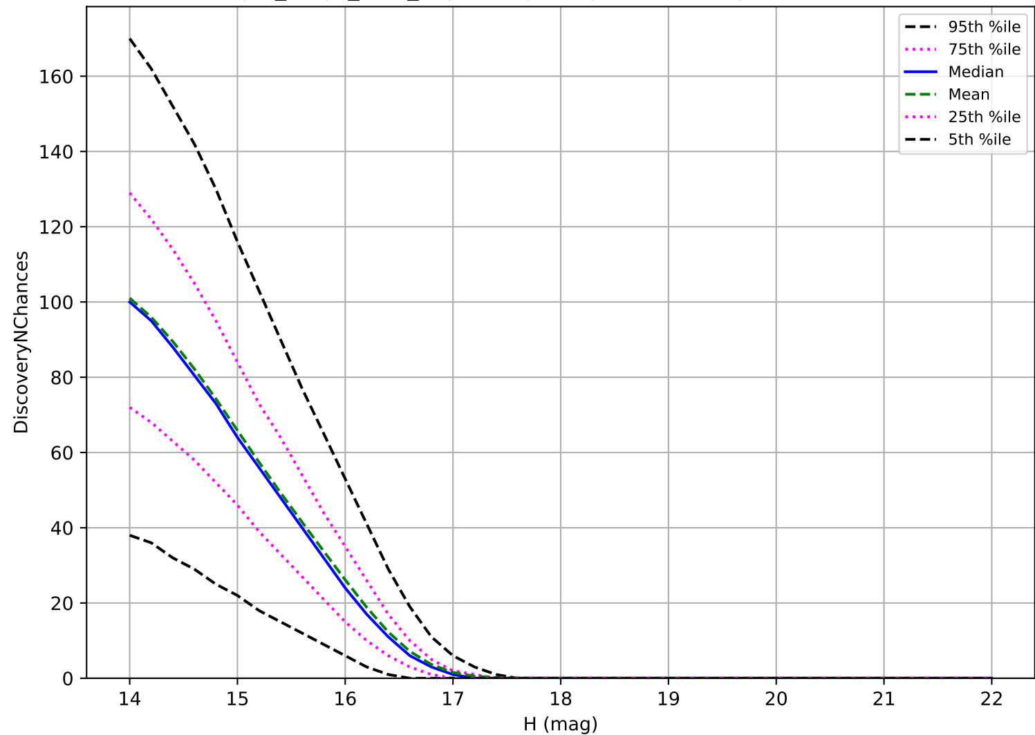
reweight_bulge_v3.3_10yrs: Trojan 3 pairs in 15 nights detection loss
