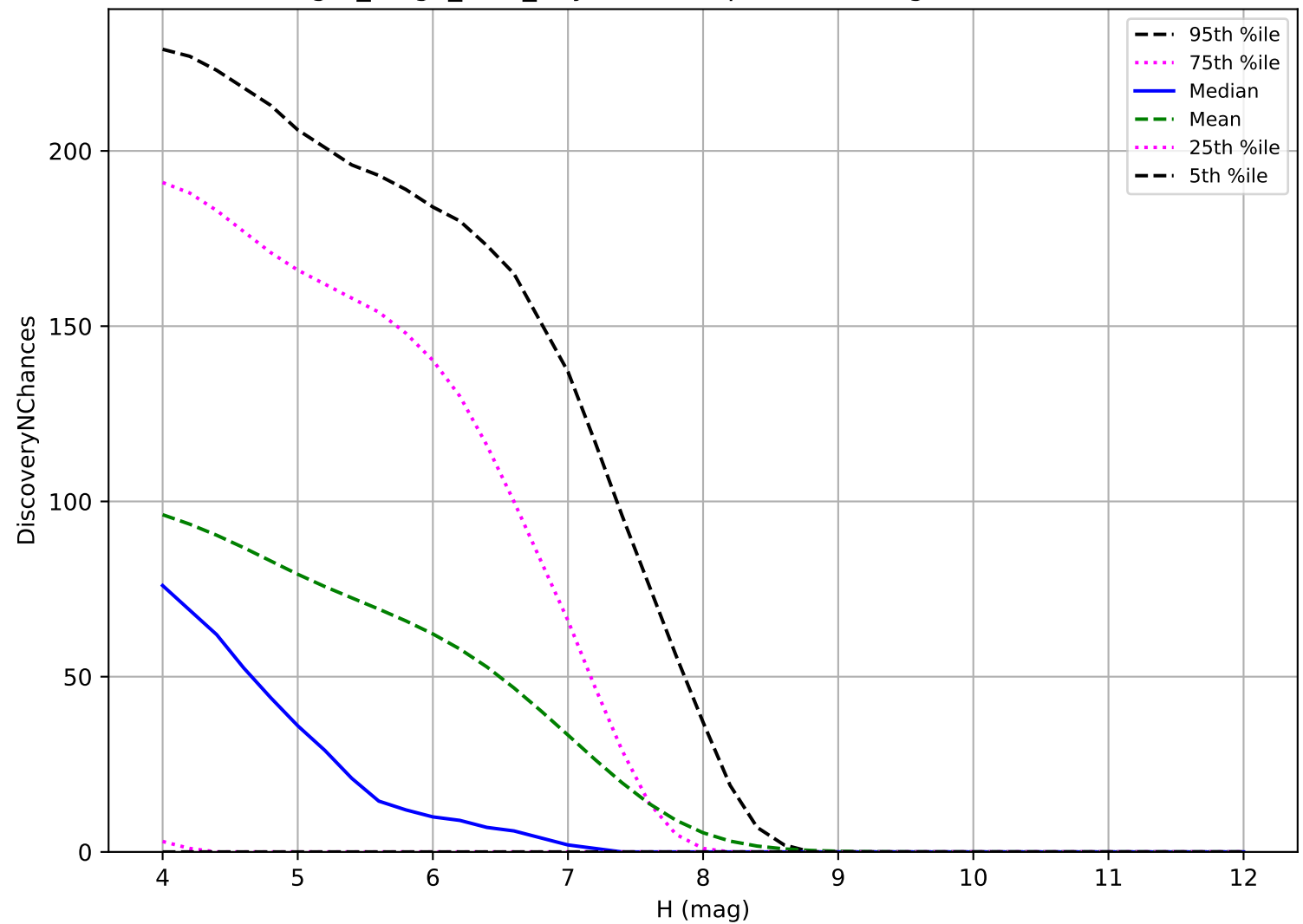
reweight_bulge_v3.3_10yrs: TNO 3 pairs in 15 nights detection loss
