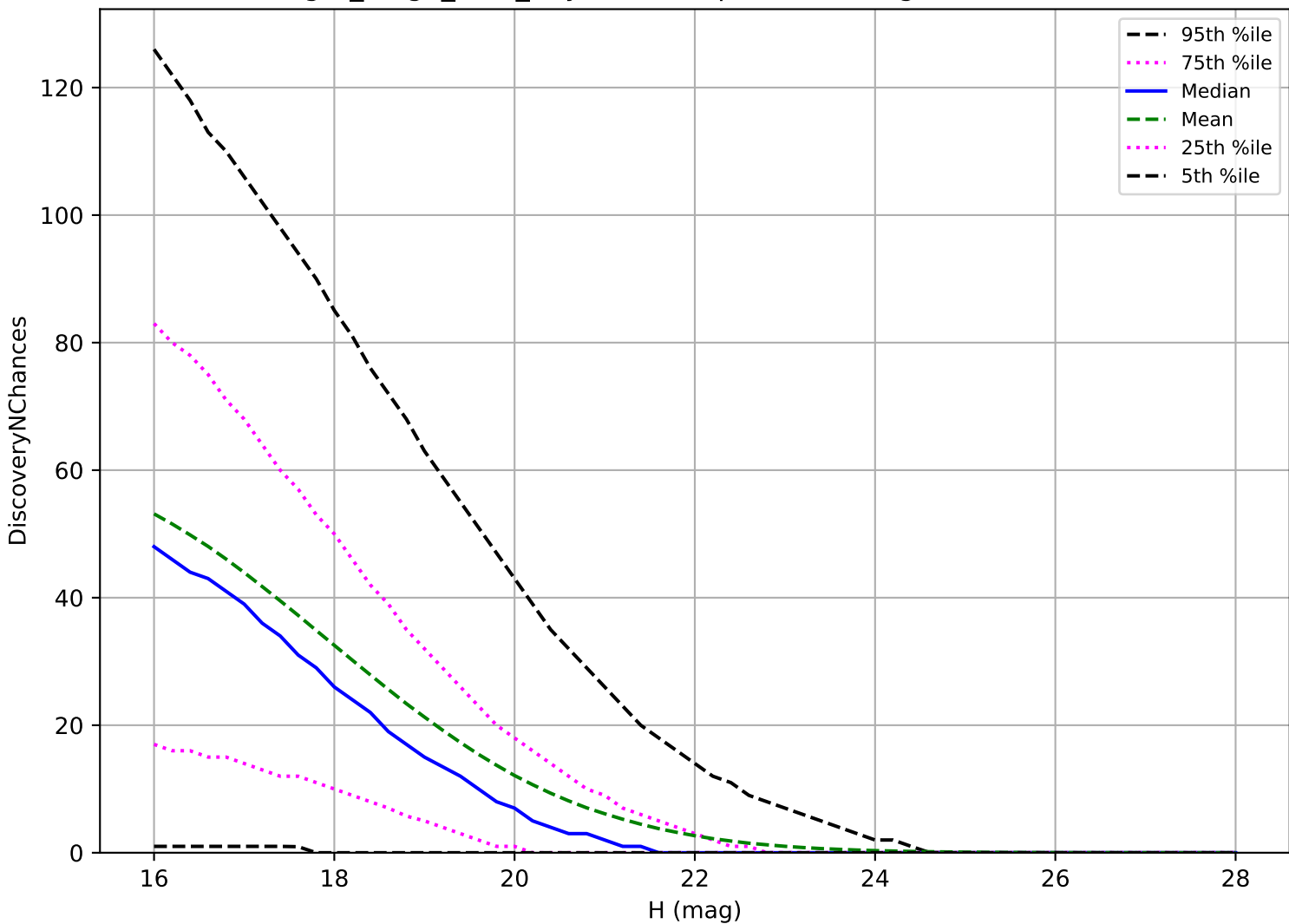
reweight_bulge_v3.3_10yrs: PHA 3 pairs in 15 nights detection loss
