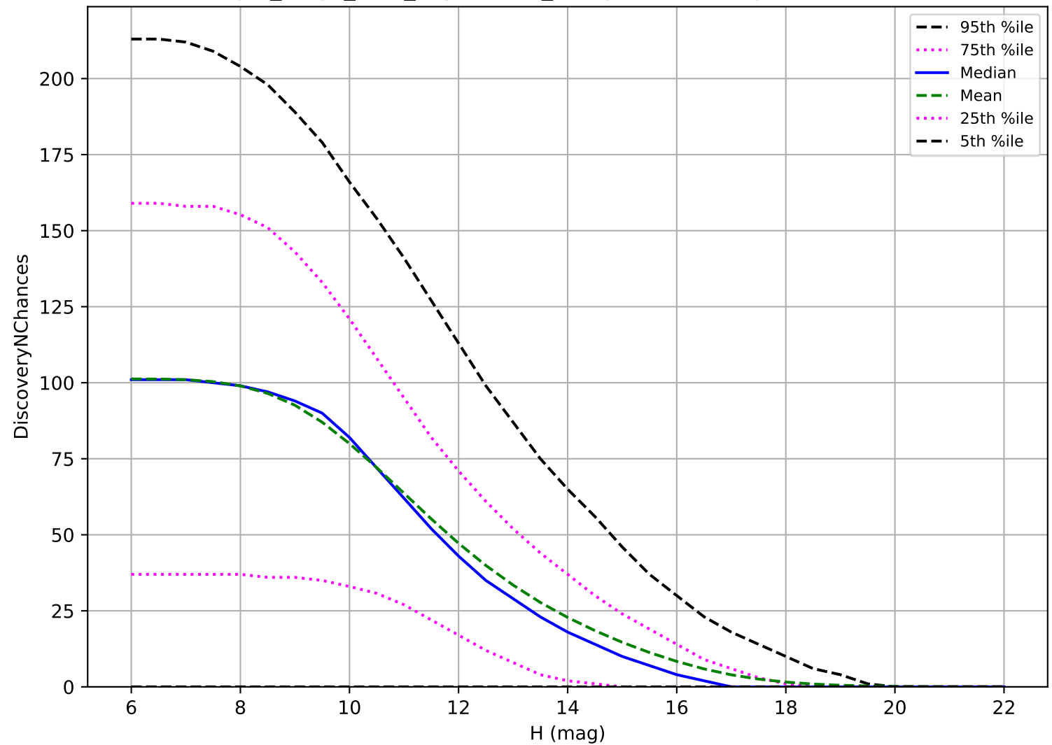
reweight_bulge_v3.3_10yrs: OCC_r5 3 pairs in 15 nights detection loss
