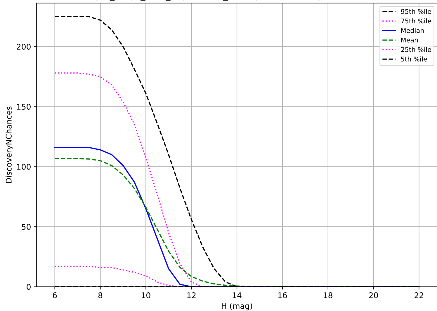
reweight_bulge_v3.3_10yrs: OCC_r20 3 pairs in 15 nights detection loss
