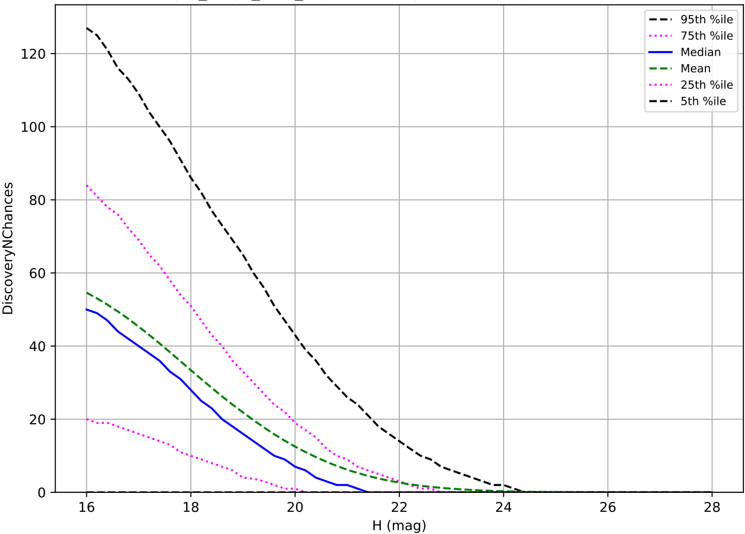
reweight_bulge_v3.3_10yrs: NEO 3 pairs in 15 nights detection loss
