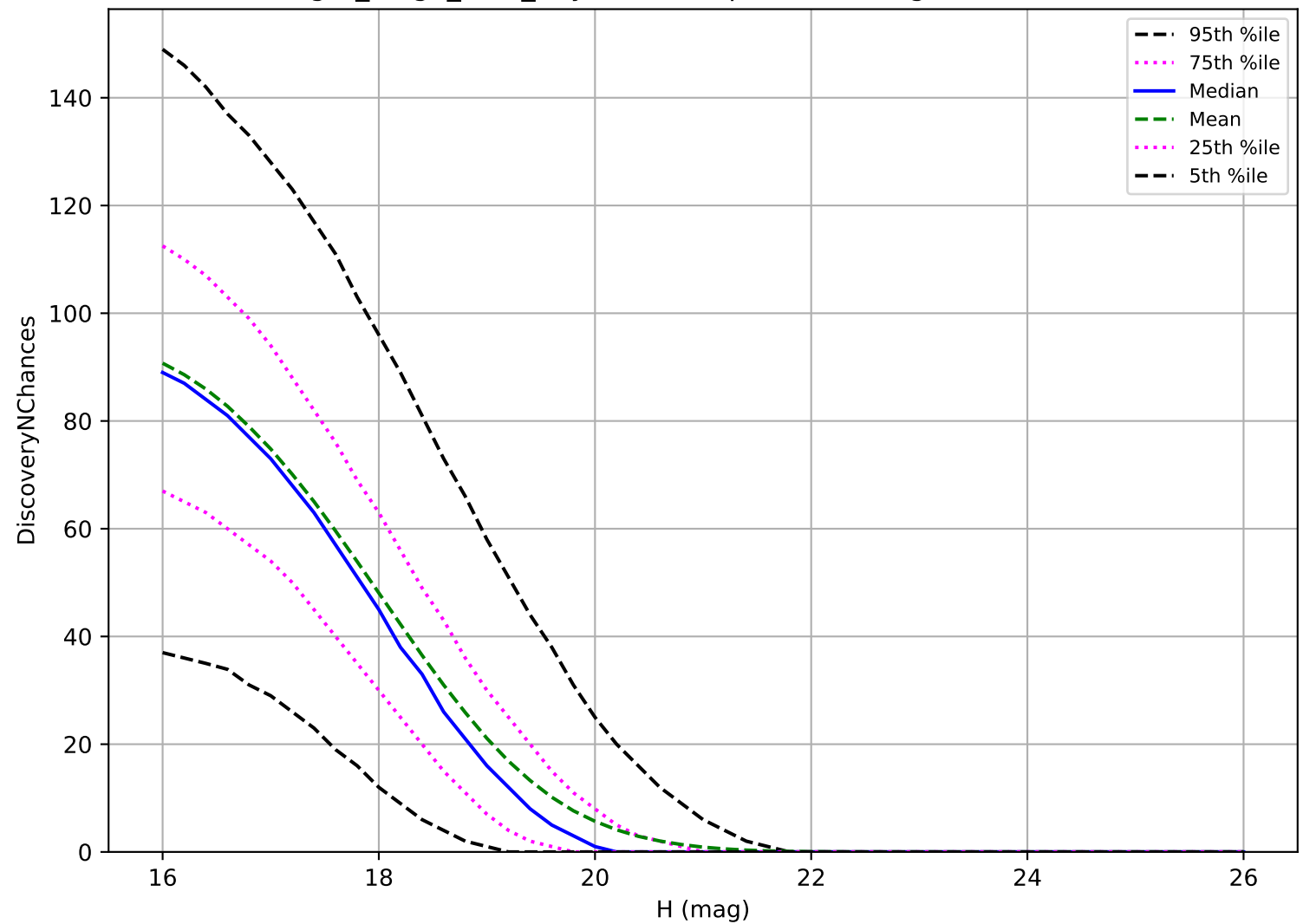
reweight_bulge_v3.3_10yrs: MBA 3 pairs in 15 nights detection loss
