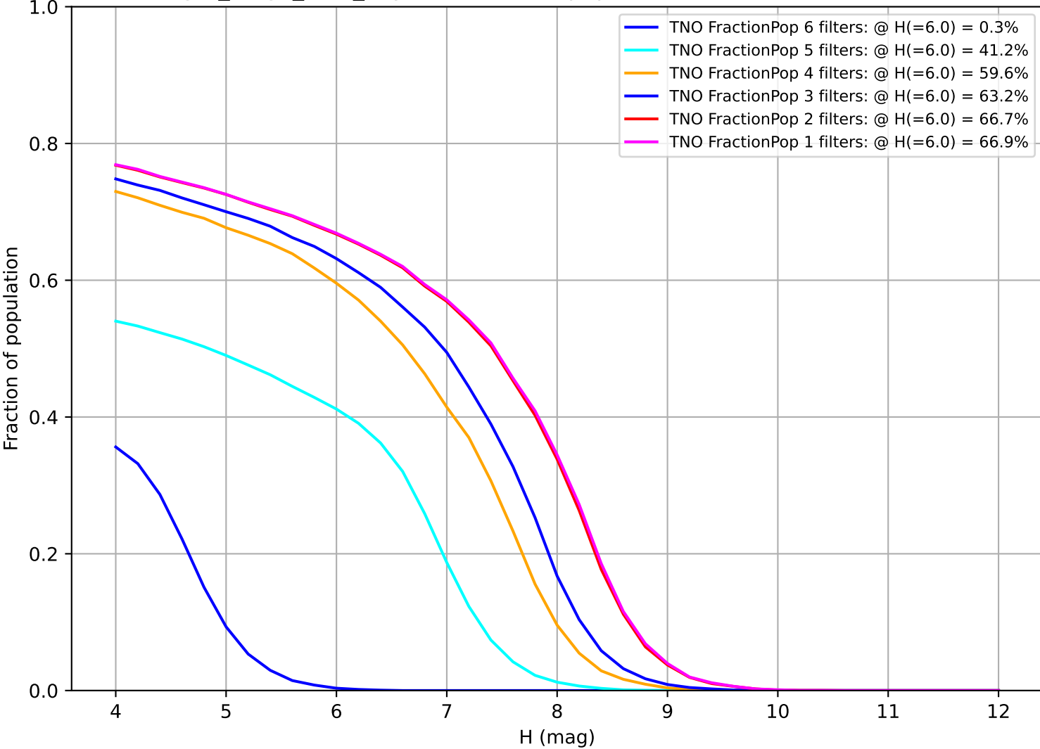
reweight_bulge_v3.3_10yrs: Fraction of population with colors in X filters TNO
