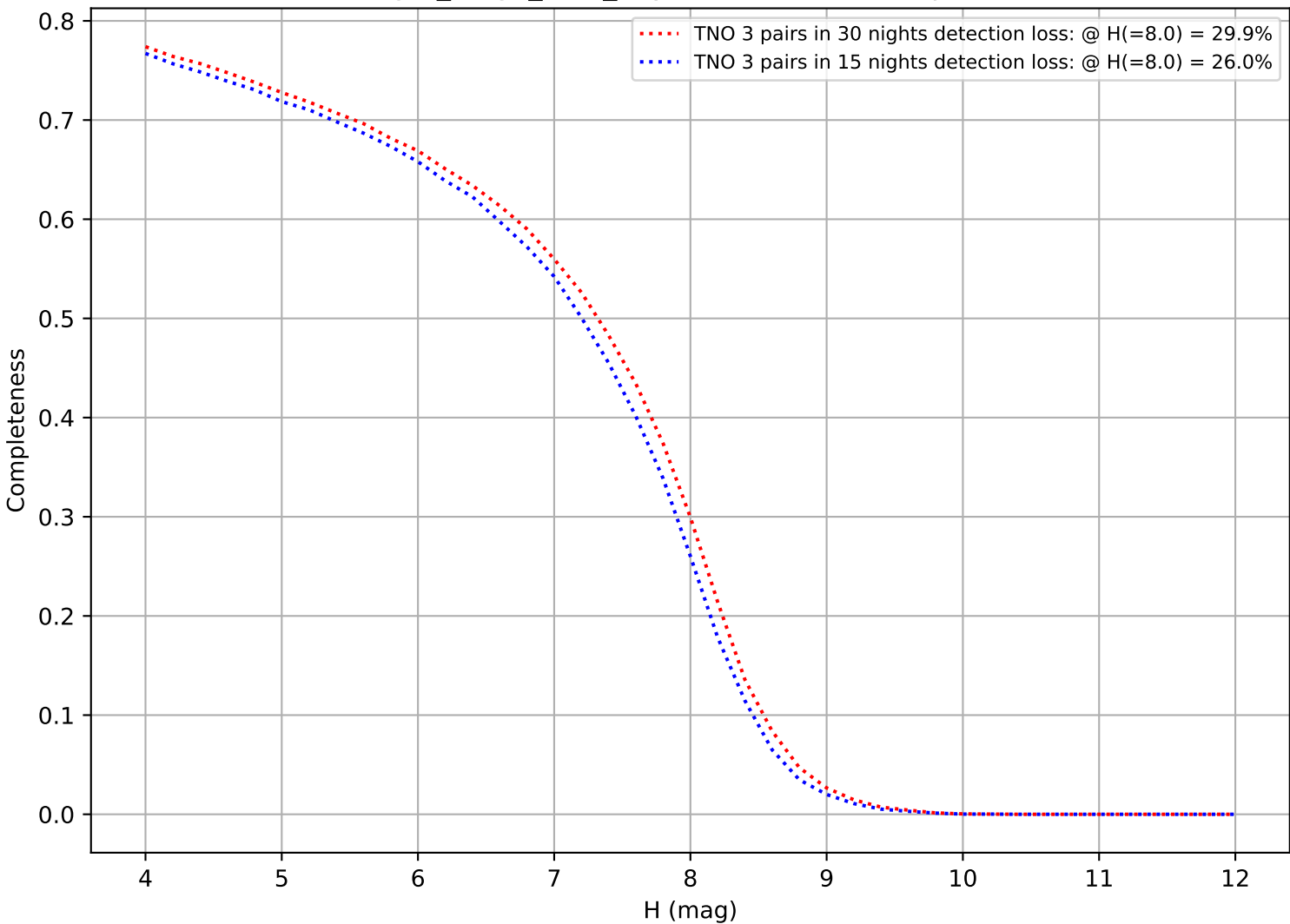
reweight_bulge_v3.3_10yrs: DifferentialCompleteness
