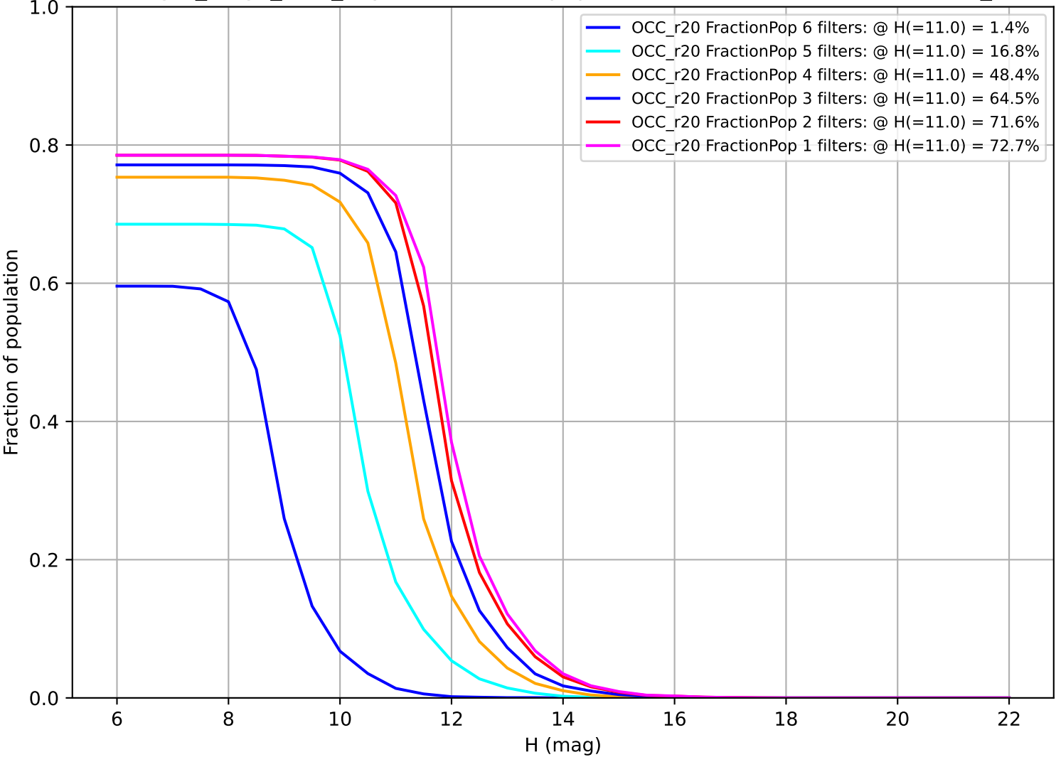
reweight_bulge_v3.3_10yrs: Fraction of population with colors in X filters OCC_r20
