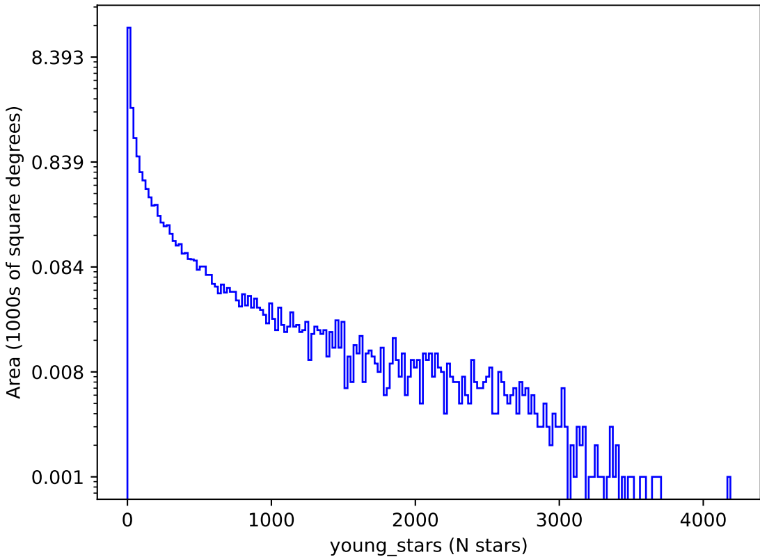
reweight_bulge_v3.3_10yrs : young_stars
