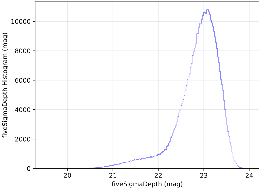
reweight_bulge_v3.3_10yrs z: fiveSigmaDepth Histogram
