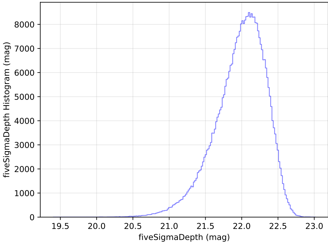
reweight_bulge_v3.3_10yrs y: fiveSigmaDepth Histogram
